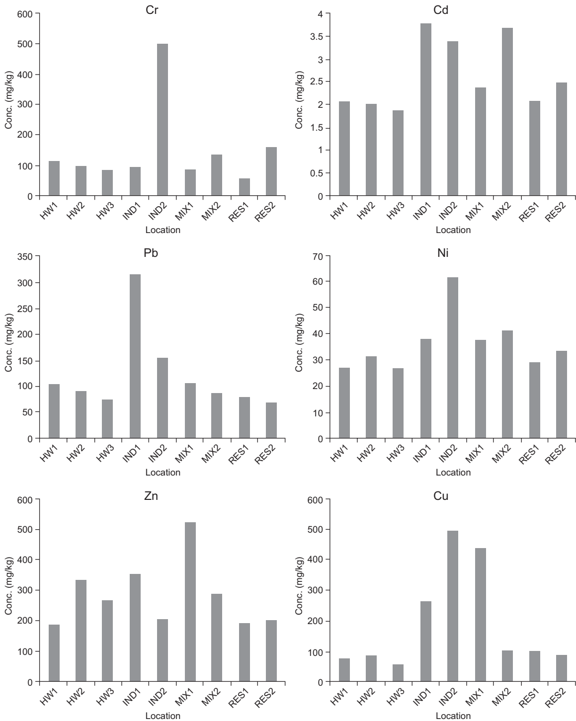
Fig. 2. Metal concentrations in road dust samples in Delhi. Concentration values of Cr, Pb, Ni, Zn and Cu for HW1, HW2, HW3, IND1, IND2, MIX2 and RES2 are taken from Rajaram et al. (2014).
